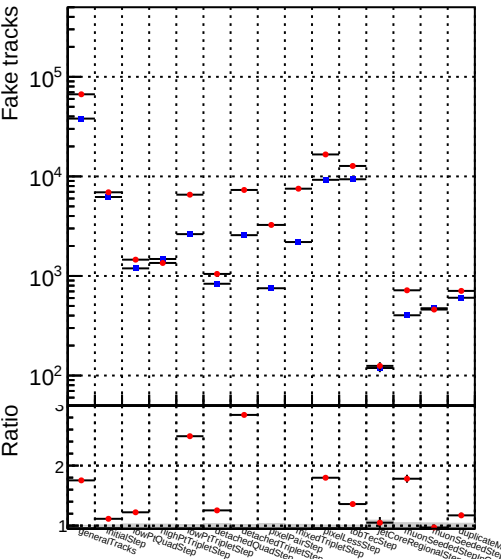
Number —●— DQM_DisplacedSUSY_mkFit_BDT
