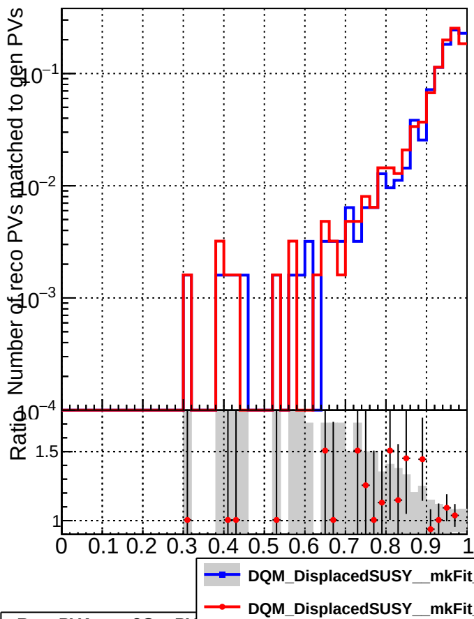
RecoPVAssoc2GenPVmatched_missing
