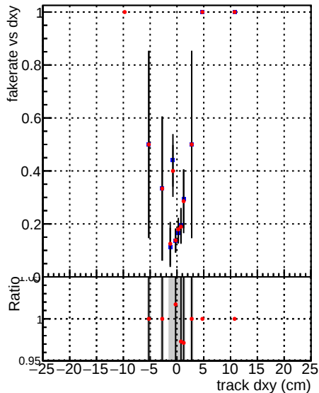
—●— DQM_DisplacedSUSY_mkFit —●— DQM_DisplacedSUSY_mkFit_BDT
