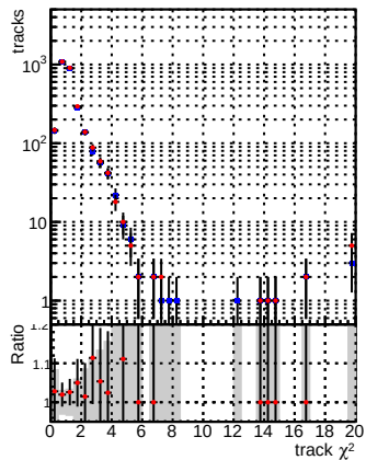
N of reco track vs. —●— DQM DisplacedSUSY mkFit —●— DQM DisplacedSUSY mkFit BDT
