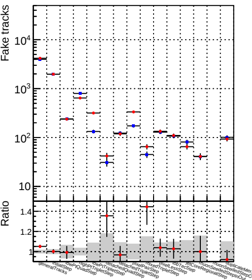
Number 1 DQM_DisplacedSUSY__mkFit_BDT_
