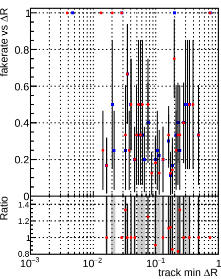
Legend: DQM_DisplacedSUSY_mkFit_ (blue dots), DQM_DisplacedSUSY_mkFit_BDT_ (red dots)
