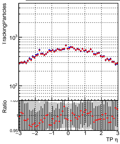
Legend: DQM_DisplacedSUSY_mkFit_ (blue stars), DQM_DisplacedSUSY_mkFit_BDT_ (red stars)
