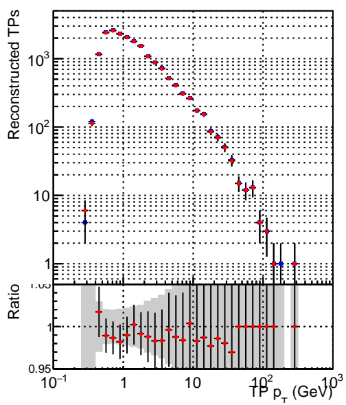
Legend: DQM_DisplacedSUSY_mkFit_ (blue stars), DQM_DisplacedSUSY_mkFit_BDT_ (red stars)
