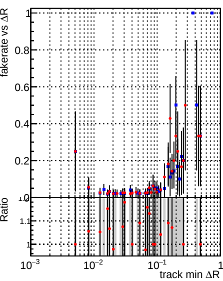
Legend: DQM_DisplacedSUSY_mkFit_ (blue line with error bars), DQM_DisplacedSUSY_mkFit_BDT_ (red line with error bars)
