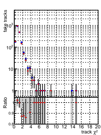
Legend: DQM_DisplacedSUSY_mkFit (blue circles), DQM_DisplacedSUSY_mkFit_BDT_ (red circles)
