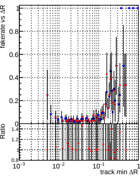
Legend: DQM_DisplacedSUSY_mkFit_ (blue squares), DQM_DisplacedSUSY_mkFit_BDT_ (red circles)
