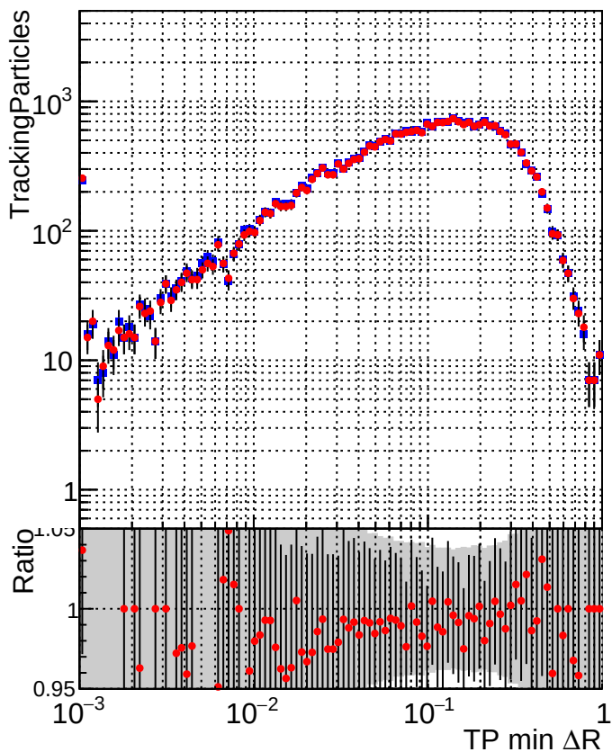
N of simulated tracks vs \Delta R
