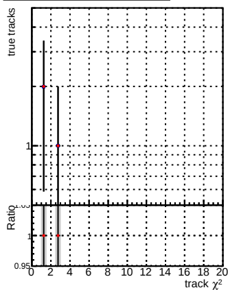
N of associated (recoToSim) tracks vs. s
