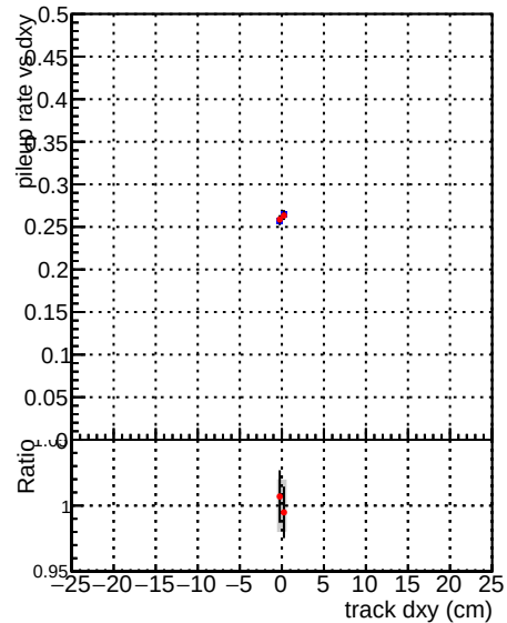
—•— DQM_DisplacedSUSY_mkFit —•— DQM_DisplacedSUSY_mkFit_BDT
