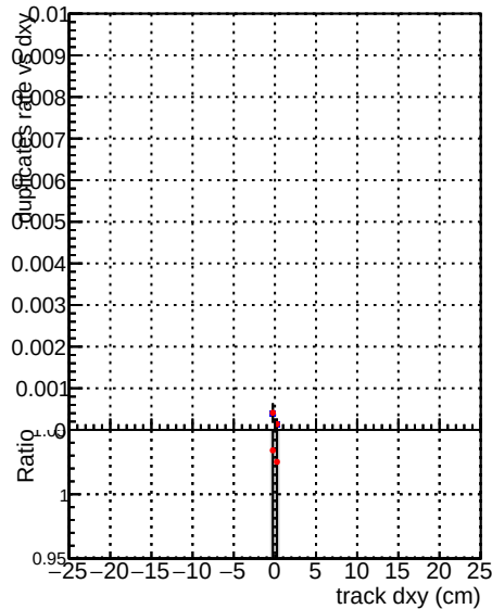
—•— DQM_DisplacedSUSY_mkFit —•— DQM_DisplacedSUSY_mkFit_BDT
