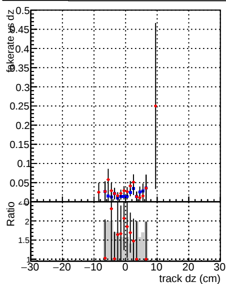
—•— DQM_DisplacedSUSY_mkFit —•— DQM_DisplacedSUSY_mkFit_BDT
