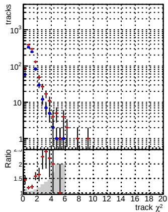
Legend: - DQM_DisplacedSUSY_mkFit (blue circles) - DQM_DisplacedSUSY_mkFit_BDT_ (red circles)
