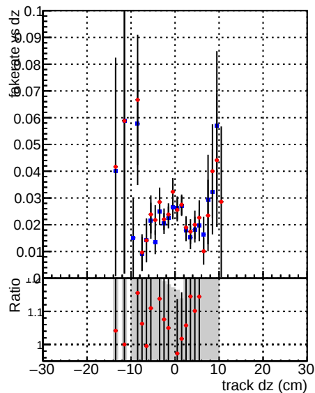
—●— DQM_DisplacedSUSY_mkFit —●— DQM_DisplacedSUSY_mkFit_BDT
