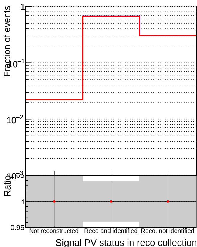
TruePVLocationIndexInRecoVertexCollectionCumulative
