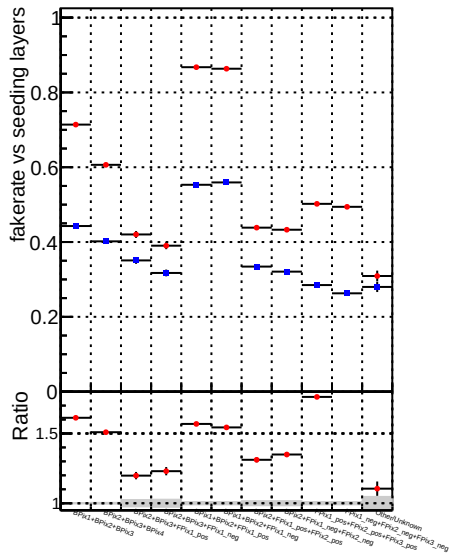
Fake rate vs. seedings
