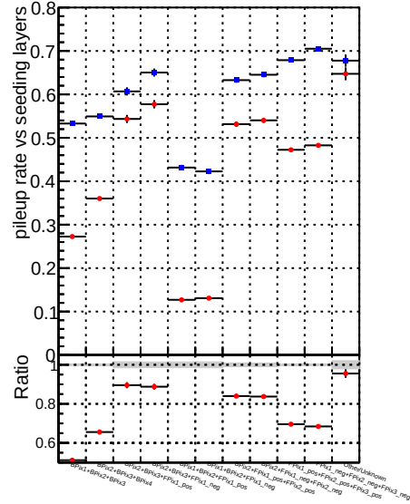
Pileup rate vs seedings
