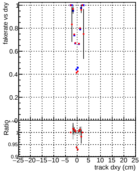
—●— DQM_DisplacedSUSY_mkFit —●— DQM_DisplacedSUSY_mkFit_BDT
