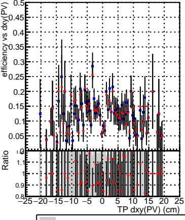
Efficiency vs DQM_DisplacedSUSY_mkFit_BDT
