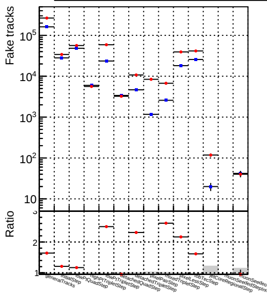
Number —●— DOM DisplacedSUSY mkFit BDT
