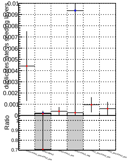
Duplicates Rate vs seeding layers
