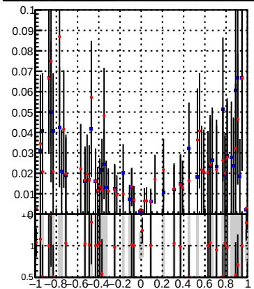
Efficiency vs Dxy(PV) for DQM_DisplacedSUSY_mkFit_ and DQM_DisplacedSUSY_mkFit_BDT_
