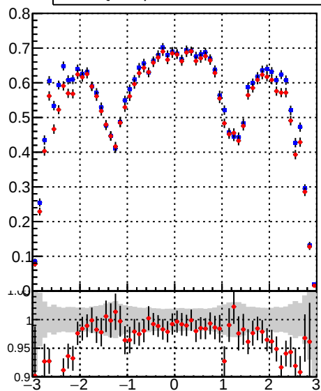
\text{DQM\_DisplacedSUSY\_mkFit\_} \text{DQM\_DisplacedSUSY\_mkFit\_BDT\_}
