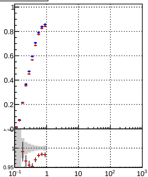
\text{DQM\_DisplacedSUSY\_mkFit\_} \text{DQM\_DisplacedSUSY\_mkFit\_BDT\_}
