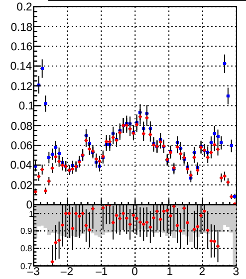
—■— DQM_DisplacedSUSY_mkFit_ —●— DQM_DisplacedSUSY_mkFit_BDT_
