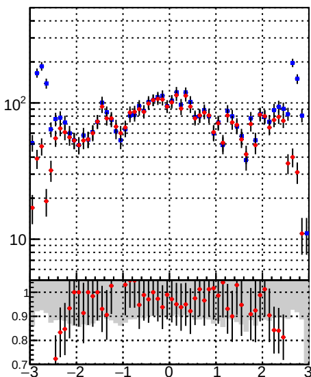
—•— DQM_DisplacedSUSY__mkFit_ —•— DQM_DisplacedSUSY__mkFit_BDT_ N of simulated tracks vs phi
