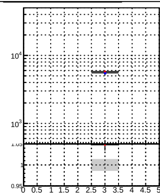
edSUSY__mkFit_BDT_
