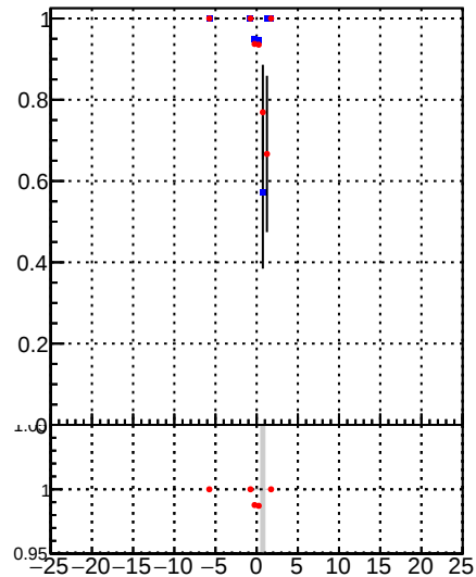
Fake rate vs d — DQM_DisplacedSUSY_mkFit — DQM_DisplacedSUSY_mkFit_BDT
