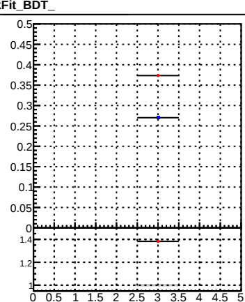
Legend: DQM_DisplacedSUSY_mkFit_ (blue), DQM_DisplacedSUSY_mkFit_BDT_ (red)
