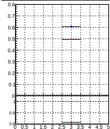
Legend: DQM_DisplacedSUSY_mkFit_ (blue), DQM_DisplacedSUSY_mkFit_BDT_ (red)
