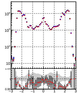
N of reco track vs \eta DQM_DisplacedSUSY_mkFit DQM_DisplacedSUSY_mkFit_BDT \eta eta
