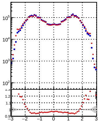
—•— DQM_DisplacedSUSY_mkFit - - - DQM_DisplacedSUSY_mkFit_BDT
