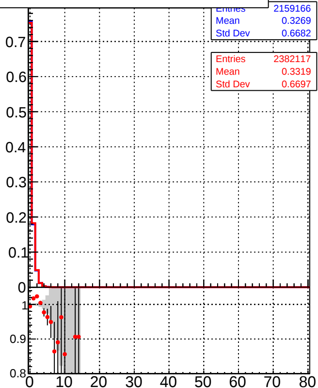
Legend for the bottom row plots: DQM_DisplacedSUSY_mkFit_ (Blue line with squares) DQM_DisplacedSUSY_mkFit_BDT_ (Red line with circles)
