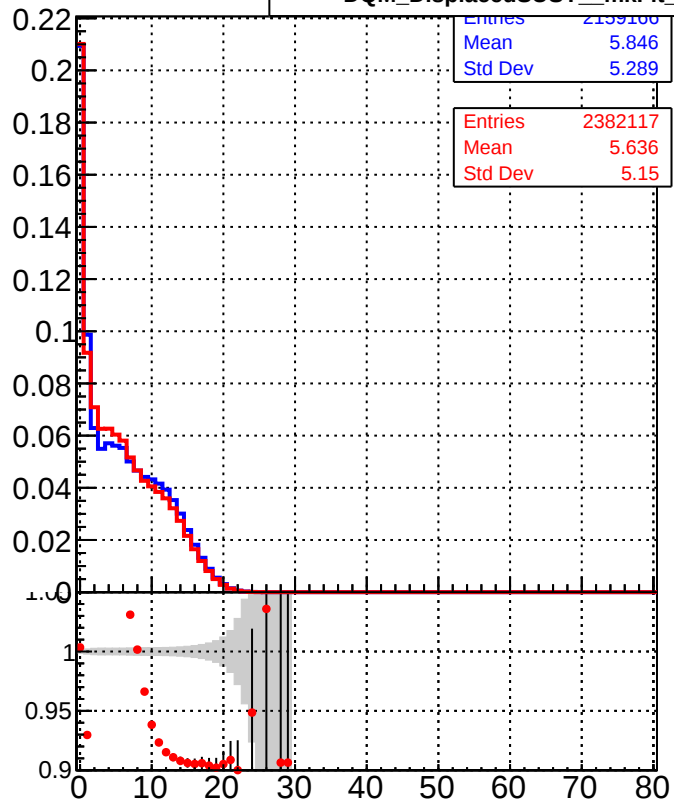
Legend for the bottom row plots: DQM_DisplacedSUSY_mkFit_ (Blue line with squares) DQM_DisplacedSUSY_mkFit_BDT_ (Red line with circles)
