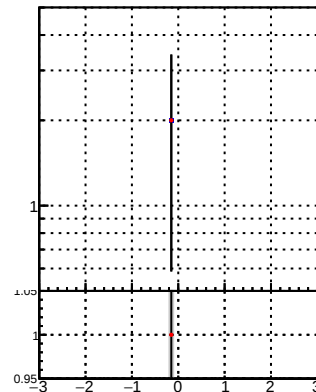
—●— DQM_DisplacedSUSY_mkFit —●— DQM_DisplacedSUSY_mkFit_BDT_
