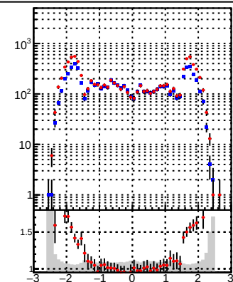
N of reco track vs \eta pT eta Legend: —♦— DQM_DisplacedSUSY_mkFit —+— DQM_DisplacedSUSY_mkFit_BDT
