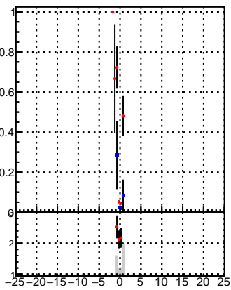
Fake rate vs dxypv
