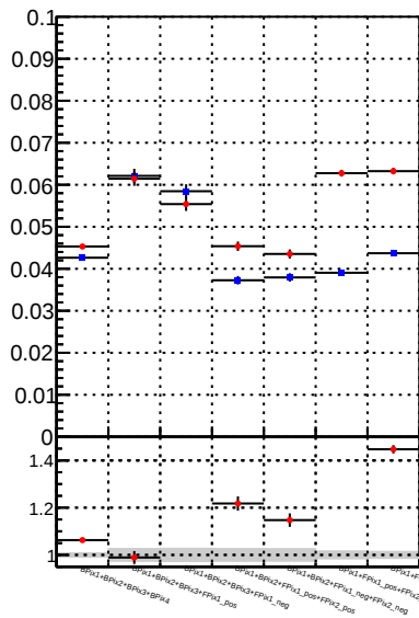
Fake rate vs. \bullet DQM_DisplacedSUSY_mkFit \bullet DQM_DisplacedSUSY_mkFit_BDT
