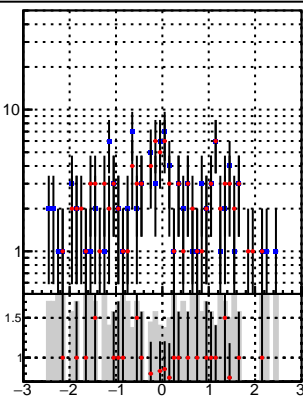
N of associated (recoToSim) tracks vs phi
