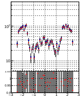
N of reco track vs \eta pT eta ● DQM_DisplacedSUSY_mkFit + DQM_DisplacedSUSY_mkFit_BDT
