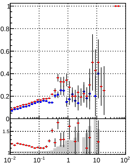
■ DQM_DisplacedSUSY_mkFit_ ■ DQM_DisplacedSUSY_mkFit_BDT_ Fake rate vs v
