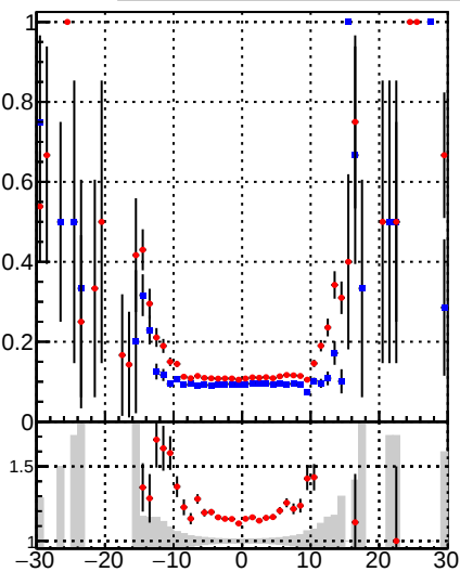
■ DQM_DisplacedSUSY_mkFit_ ■ DQM_DisplacedSUSY_mkFit_BDT_ Fake rate vs v
