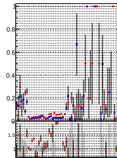
Fake rate vs. —●— DQM_DisplacedSUSY_mkFit —●— DQM_DisplacedSUSY_mkFit_BDT
