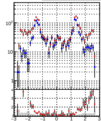
N of reco track vs \eta pT eta Legend: DQM_DisplacedSUSY_mkFit (blue line with markers) DQM_DisplacedSUSY_mkFit_BDT (red line with markers)
