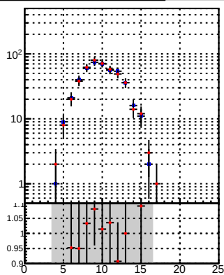
edSUSY__mkFit_BDT_
