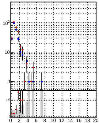
N of reco track vs. \chi^2 for DQM DisplacedSUSY mkFit and DQM DisplacedSUSY mkFit_BDT
