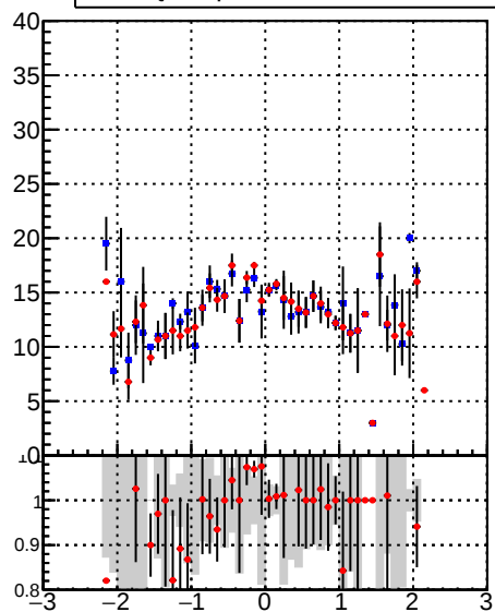
mean hit Legend: —•— DQM_DisplacedSUSY_mkFit_ —•— DQM_DisplacedSUSY_mkFit_BDT_
