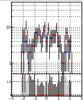
N of reco track vs \eta DQM_DisplacedSUSY_mkFit N of reco track vs \eta DQM_DisplacedSUSY_mkFit_BDT
