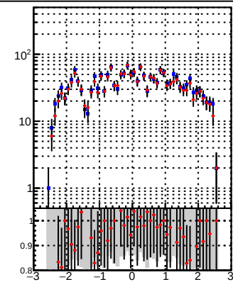
—●— DQM_DisplacedSUSY_mkFit —●— DQM_DisplacedSUSY_mkFit_BDT
