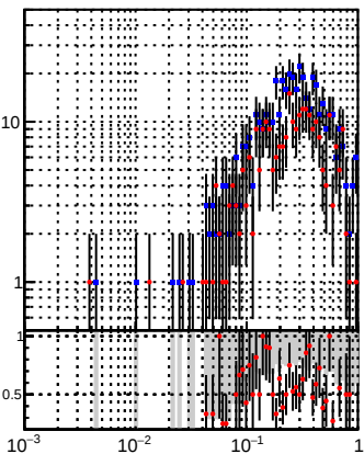
N of associated tracks (recoToSim) vs dR
