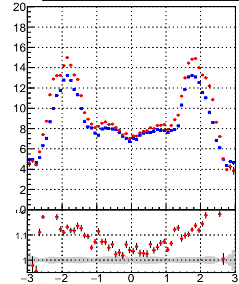
mean hit
