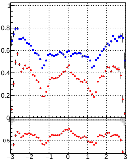
Pileup rate vs \phi
