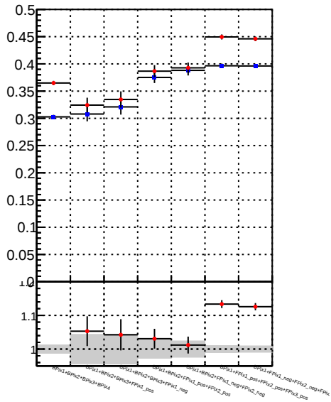
Fake rate vs. —•— DQM_DisplacedSUSY_mkFit —•— DQM_DisplacedSUSY_mkFit_BDT
